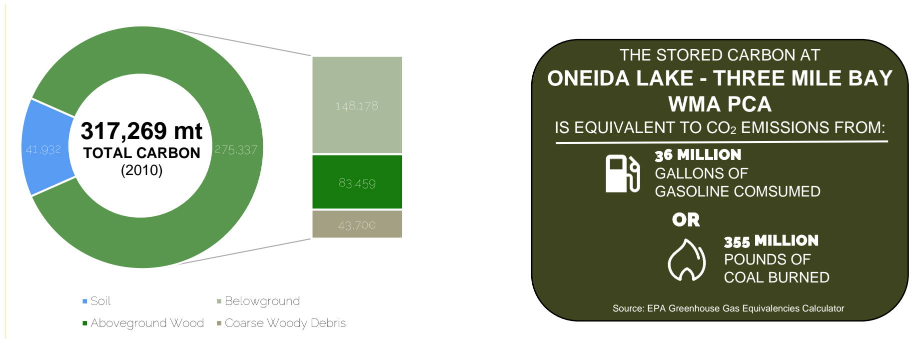
Figure 3. Sources and quantities of stored carbon at Oneida Lake - Three Mile Bay WMA PCA.
