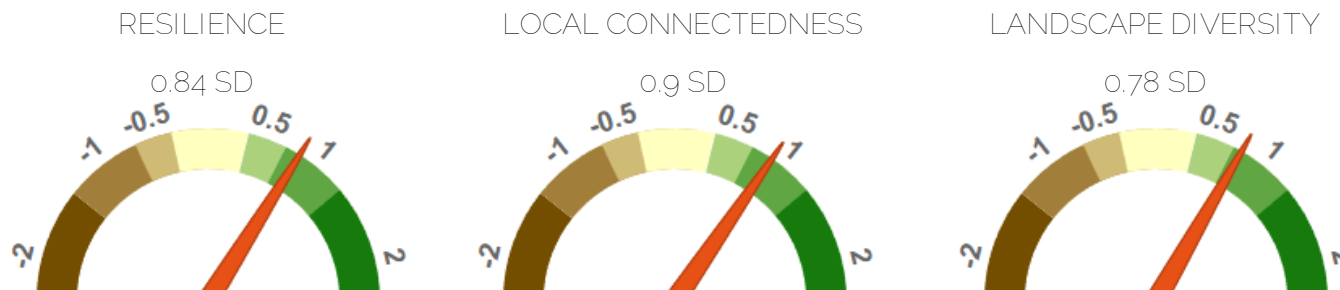
Figure 2. Site resilience, local connectedness, and landscape diversity scores for Fish Creek WMA PCA. Scores are expressed as the standard deviation above or below the average score.
