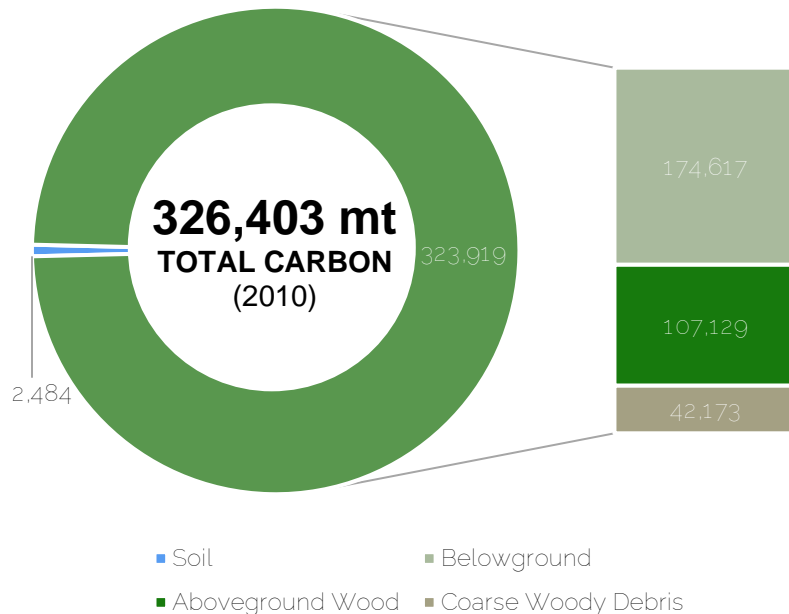
Figure 3. Sources and quantities of stored carbon at Fish Creek WMA PCA.
